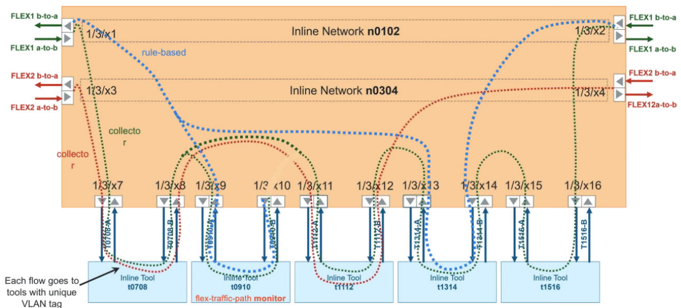
Figure 0-14: Example 6 Inline Tool Sharing by Multiple Inline Flows
