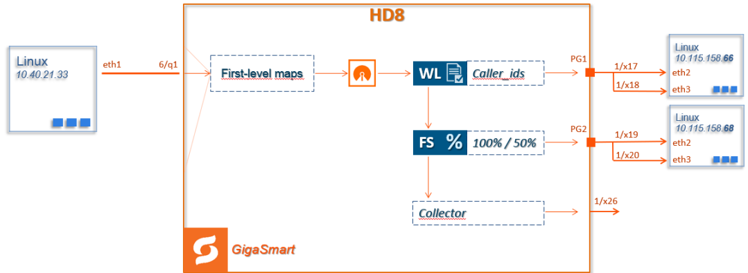
Figure 0-24: SIP/RTP Load Balancing Topology
