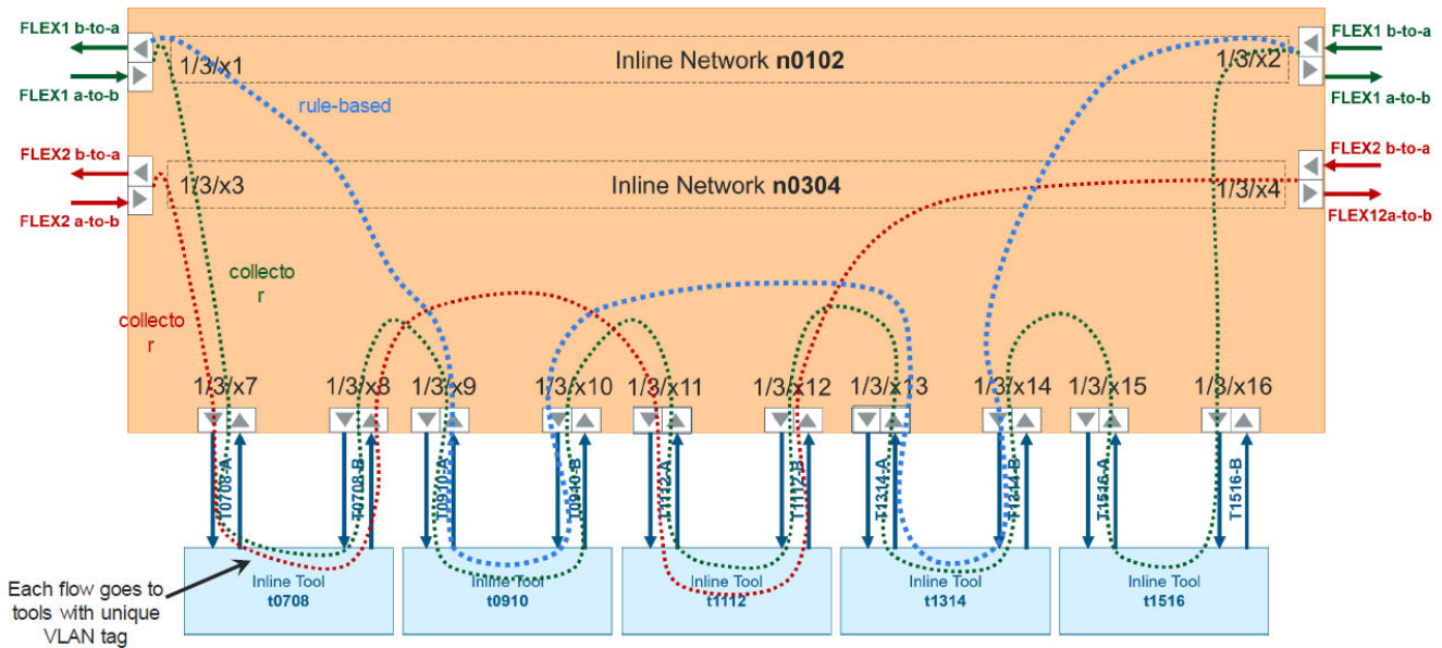
Figure 0-13: Example 4 Inline Tool Sharing by Multiple Inline Flows
