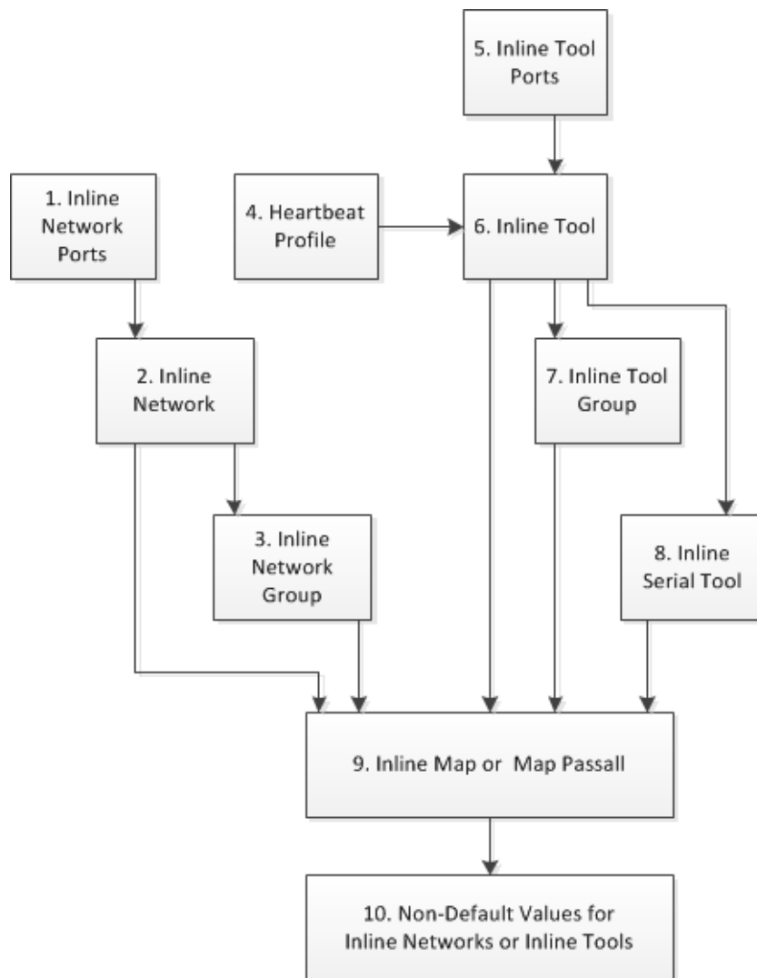
Figure 0-10: Configuration Steps for Inline Bypass Solutions
