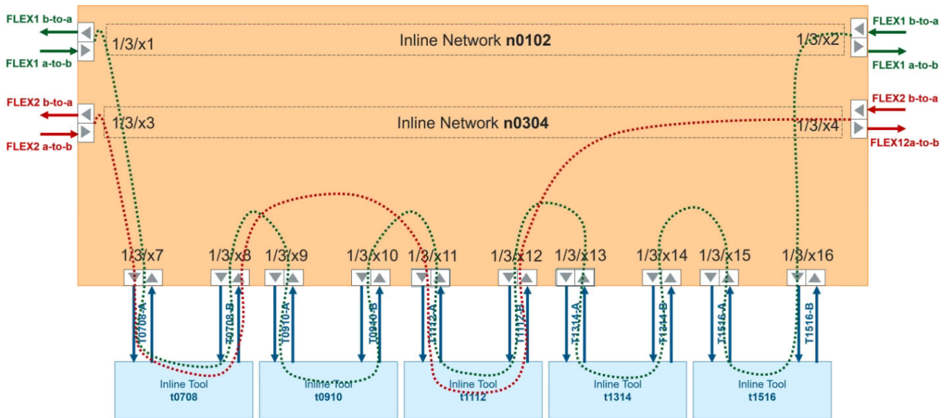
Figure 0-12: Example 2 Inline Tool Sharing by Multiple Inline Flows
